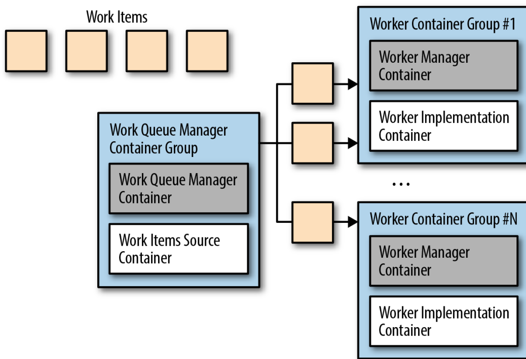
Figure 10-2. The same work queue as shown in Figure 10-1 , but this time using reusable containers. The reusable system containers are shown in white while the user-supplied container is shown in grey/blue.
