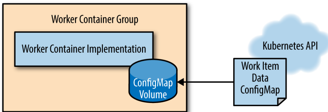
Figure 10-4. The work queue worker API
