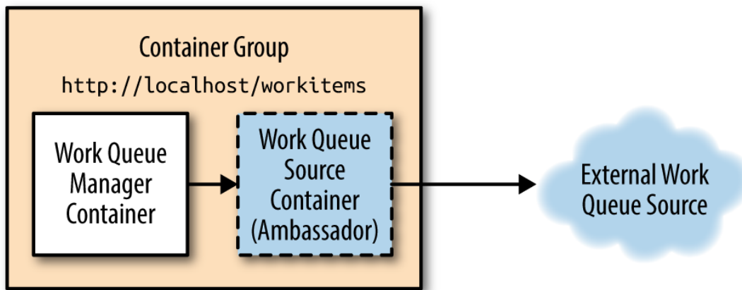
Figure 10-3. The work queue container group
